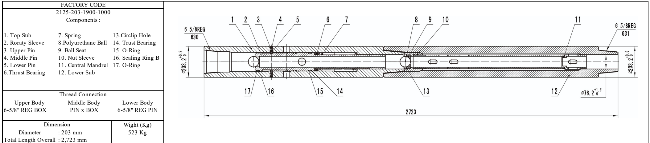
TECHNICAL DRAWING - SC-203 MULTY CIRC SUB
